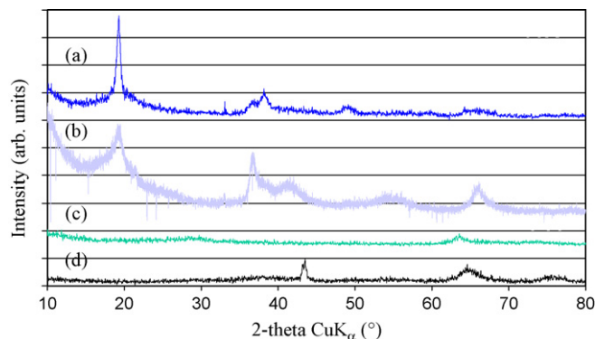
Fig. 6. Powder X-ray diffraction patterns for: (a) acid-leached \text{Li}_2\text{MnO}_3 ; 1 - x[\text{Li}(\text{Li}_{0.33}\text{Mn}_{0.67}\text{O}_2)] \cdot x[0.67\text{MnO}_2] , measured on 3/95, (b) sample from (a) measured on 10/97, (c) sample from (a) measured on 3/98, and (d), material from (a), but mixed with and in contact with carbon powder.
