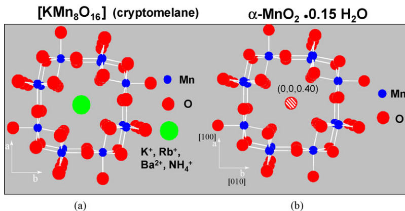
Fig. 1. Schematic structural representation of 2 \times 2 tunnel structures of MnO_2 : (a) cryptomelane, KMn_8O_{16} , and (b) hydrated \alpha\text{-MnO}_2 \cdot 0.15H_2O .
