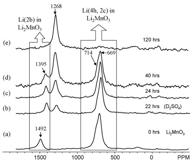
Fig. 5. Solid-state MAS Li-6 NMR of: (a) starting material \text{Li}_2\text{MnO}_3 , (b) \text{Li}_2\text{MnO}_3 after 22 h acid-leaching in 2.5 M \text{D}_2\text{SO}_4 , (c) \text{Li}_2\text{MnO}_3 after 24 h acid-leaching in 2.5 M \text{D}_2\text{SO}_4 , (d) \text{Li}_2\text{MnO}_3 after 40 h acid-leaching in 2.5 M \text{D}_2\text{SO}_4 , (e) \text{Li}_2\text{MnO}_3 after 120 h acid-leaching in 2.5 M \text{D}_2\text{SO}_4 .
