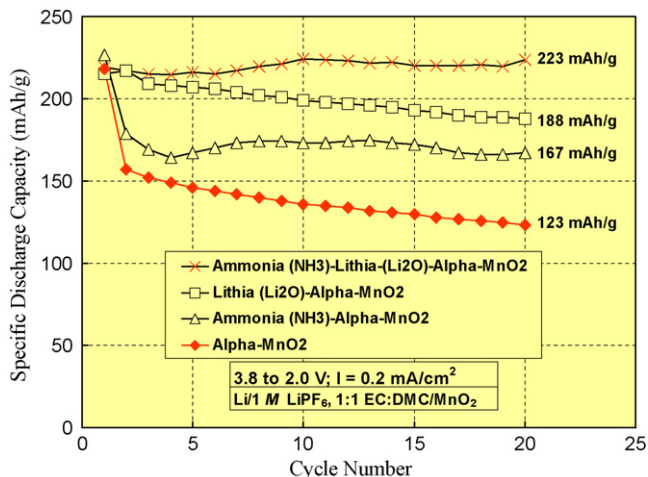
Fig. 3. Discharge capacity (mAh g -1 ) vs. cycle number for a series of \alpha -MnO 2 electrode materials.
